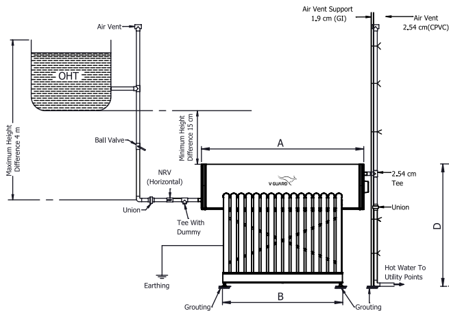
SWH System - Front View
