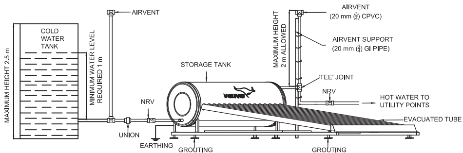
INSTALLATION DIAGRAM
